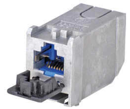
S500 CAT.6 A STP Two-Way Entry Jack CAXASM-00104-C001
